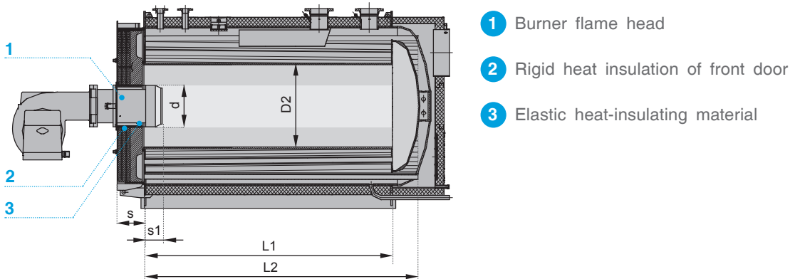
Burner installation
